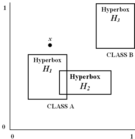
Figure 2: Learning in the FLN framework
